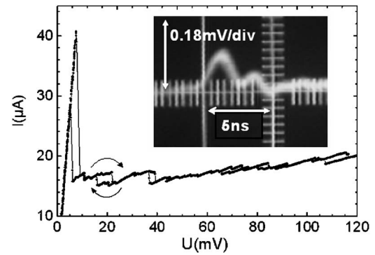
FIG. 2. Low frequency voltage-biased I V characteristics of a typical AFM-made SSPD device measured at 4.2 K. The hot-spot plateau is at 16 \mu\text{A} , one third of the value of the critical current. Inset: Oscilloscope time trace of a single count event, measured in the same condition with high frequency lines (the 75 dB amplification of the rf has been subtracted).
