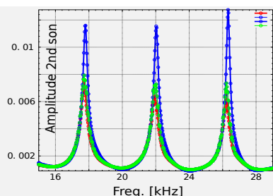
Resonance modes of a miniature 2 nd sound cavity, with a flow passing through it, and carrying many (red) or few (blue) quantum vortices.
