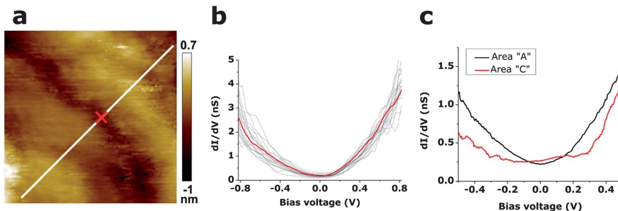
Fig. 4 Spectroscopy measurements acquired on ripples and on strain-free regions. The spectra displayed in (b) have been taken along the white line drawn on the STM image (a) ( 80 \times 80 nm 2 ). There is no significant difference between the spectra acquired on the two ripples or in between. The red cross in (a) corresponds to the position where the red spectrum displayed in (b) was measured. (c) Spatially averaged spectra acquired on strain-free graphene, far from the metallic contact (area A, black curve) and on strained graphene, close to the metallic contact (area C, red curve).
