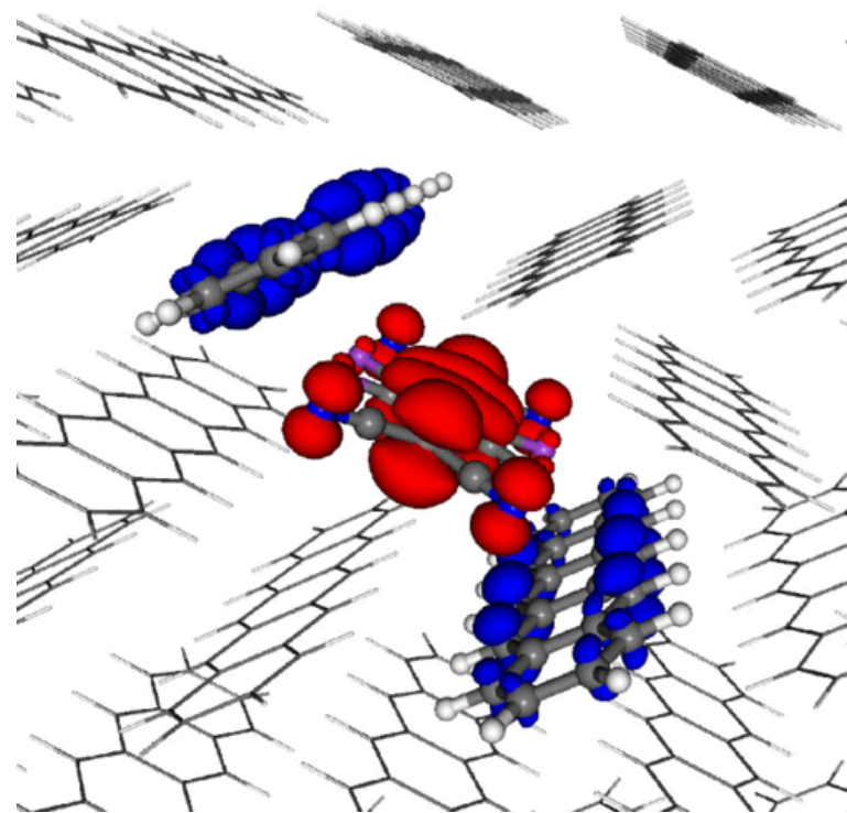
Figure : charge-transfer excitation from pentacene to F4TCNQ acceptor as given by embedded Bethe-Salpeter calculations. The associated hole-averaged electron density and electron-averaged hole density are given in red and blue, respectively. The skeleton molecules are model polarizable molecules in a QM/MM spirit. From: Li et al. Phys. Rev. Mater. 1 , 025602 (2017)
