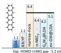
Pentacene DFT-LDA total energies (6-311G*)
